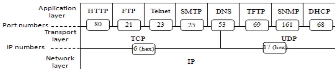
TCP ports and IP protocols numbers
